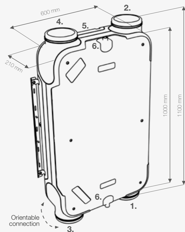
Airflow right version (factory version)
