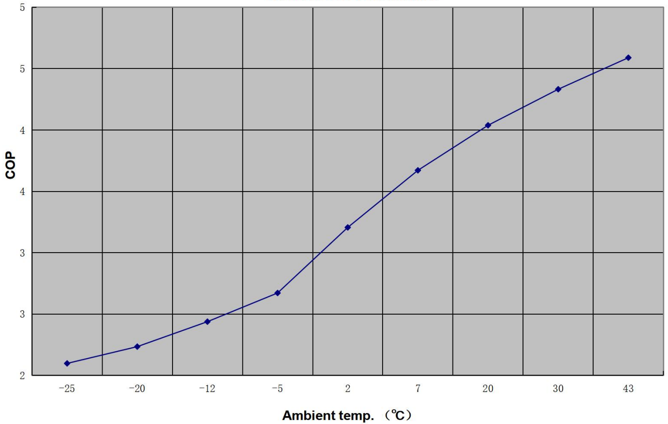
Curve of COP Performance
