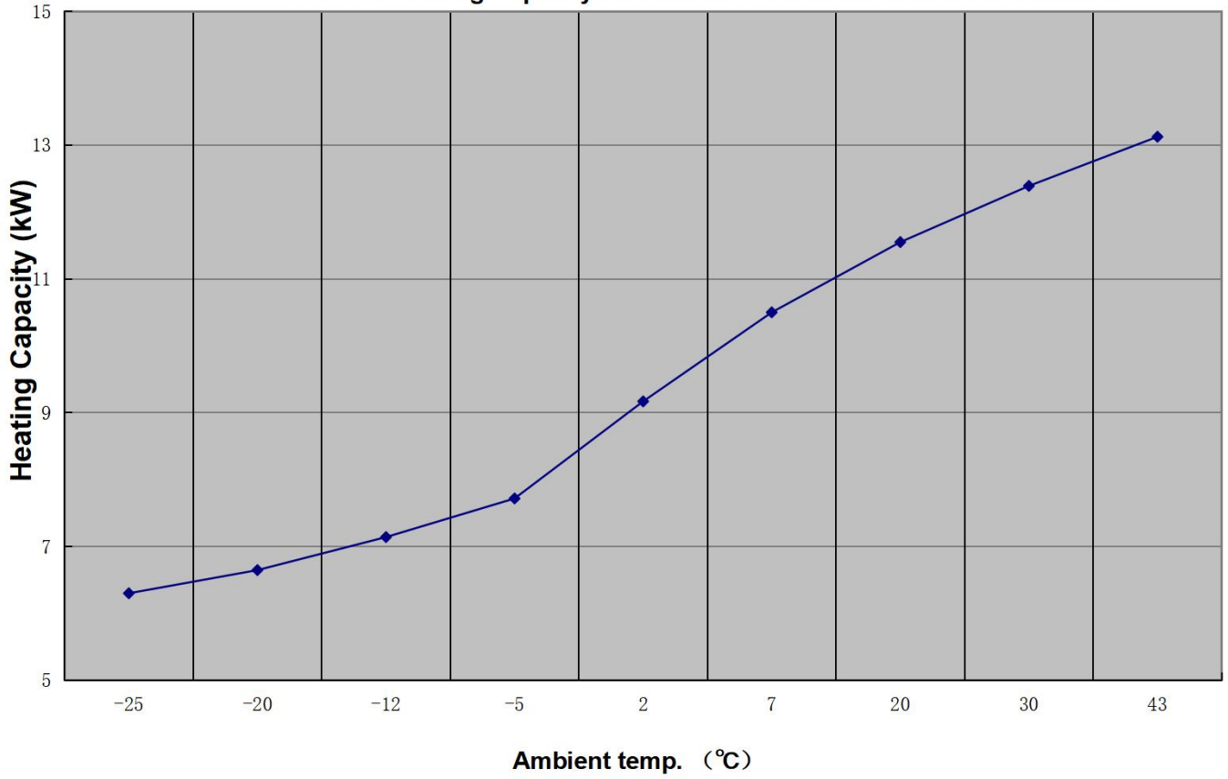
Curve of Heating Capacity Performance-3E040-DKZLRS-A for hot water
