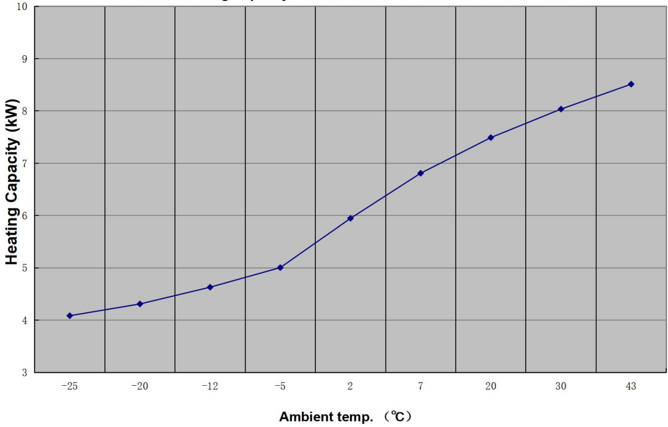
Curve of Heating Capacity Performance-3E030-DKZLRS-A for hot water
